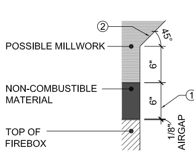
A SECTION DETAIL @ MILLWORK
