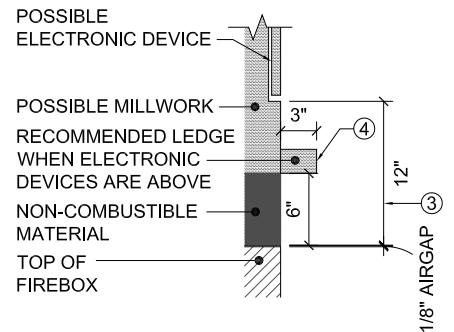
B SECTION DETAIL @ ELECTRONIC DEVICE
